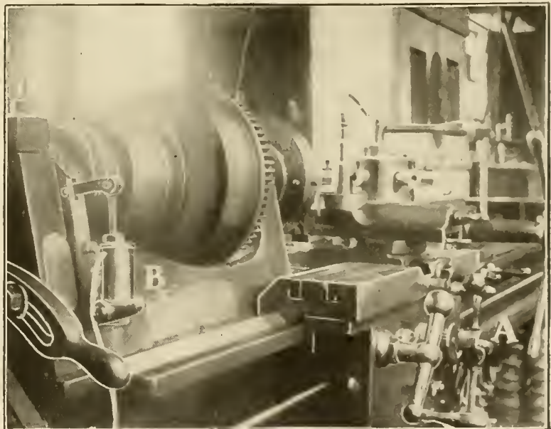
PNEUMATIC BELT SHIFTER.
